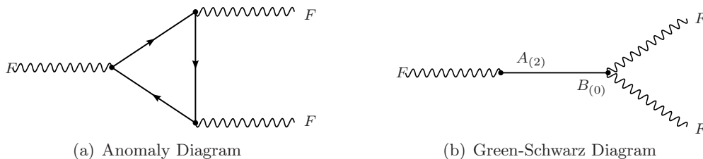
Figure 1. Anomaly and Green-Schwarz diagrams.
